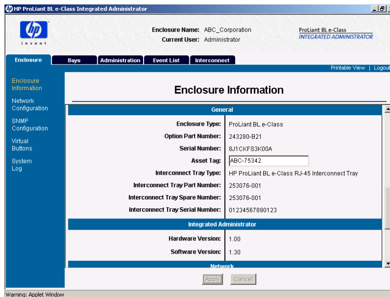
Figure 5-2: Setting the asset tag number
