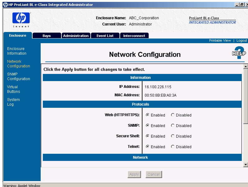
Figure 3-7: Network Configuration screen (information and protocols areas, 1 and 2 of 3, shown)
