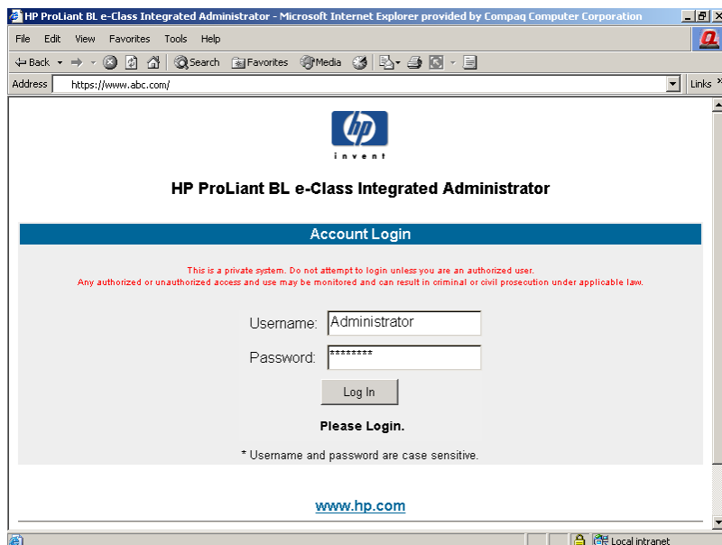
Figure 2-5: Login screen
