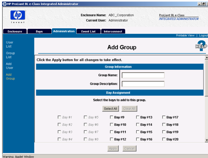
Figure 3-20: Add Group screen (Group Information and Bay Assignment areas, 1 and 2 of 3, shown)
