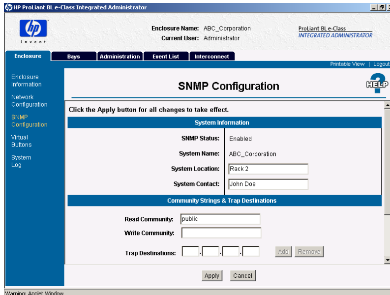
Figure 5-12: Setting a community string, trap target destinations, or system location and contact information
